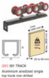
Wood Sliding Fitting Roller Set | 100kg
