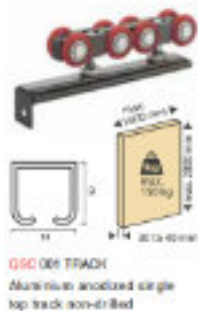
Wood Sliding Fitting Roller Set | 150kg
